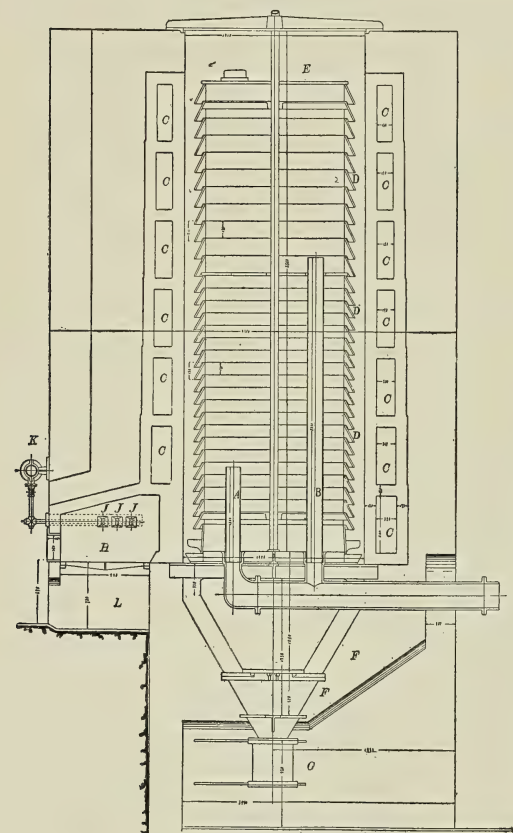
FIG. 81.—Retort for Distilling Pure Lignite.
